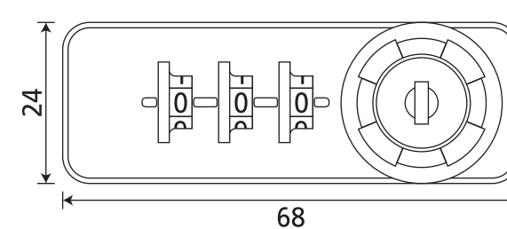
3-digit combination dial (Front:Full scale) 3桁ダイヤル錠 (表：実寸)
