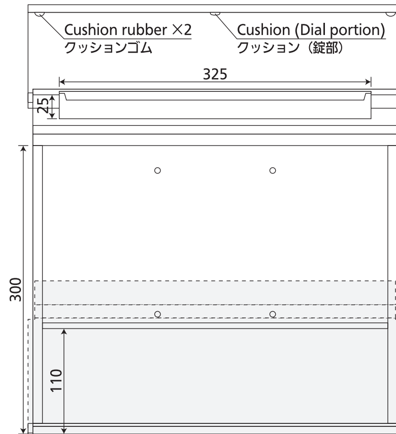
[ Front view (Opened the door) ]
